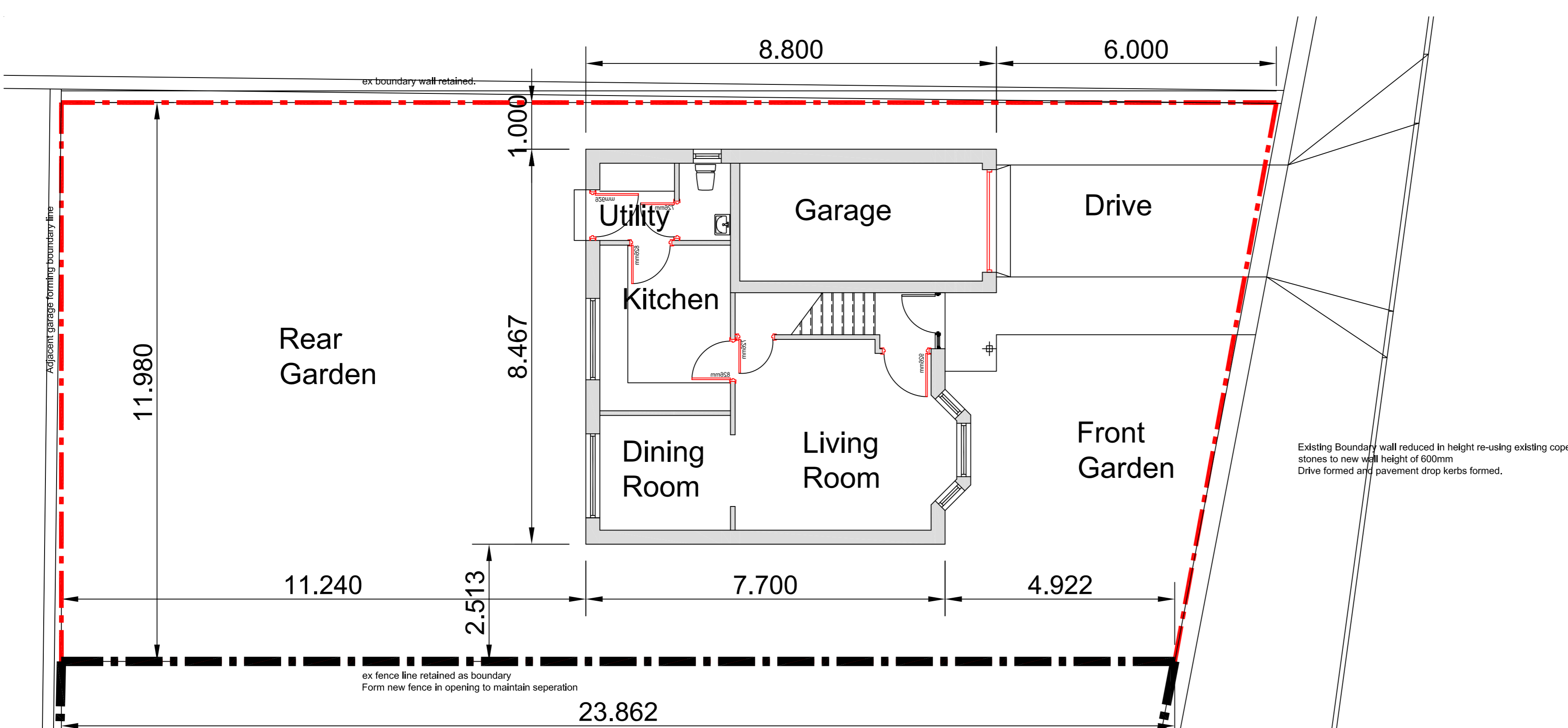
Site Layout Plan scale 1/50
