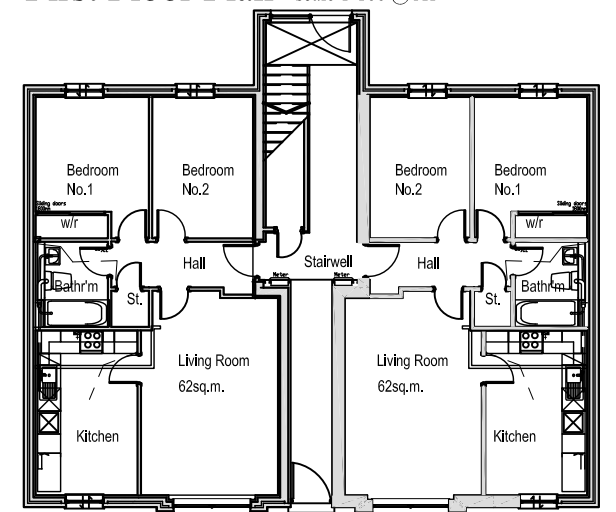
Block A Ground Floor Plan - scale 1-100 @ A1
