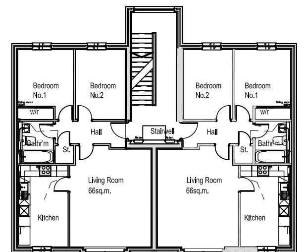
Block A First Floor Plan - scale 1-100 @ A1
