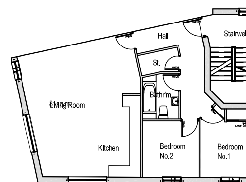
Block B First Floor Plan - scale 1-100 @ A1
