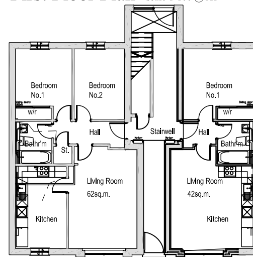
Block C Ground Floor Plan - scale 1-100 @ A1
