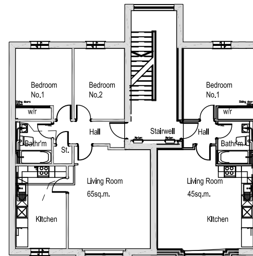
Block C First Floor Plan - scale 1-100 @ A1
