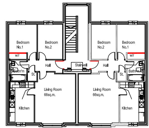
First Floor Plan - Standard Block Scale 1/100
