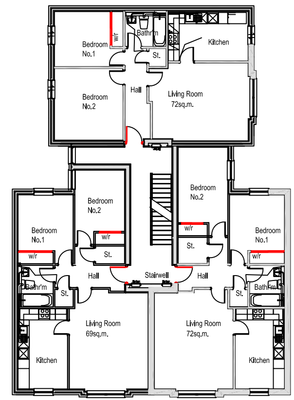
First Floor Plan - T Block Scale 1/100
