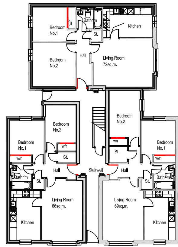
Ground Floor Plan - T Block Scale 1/100
