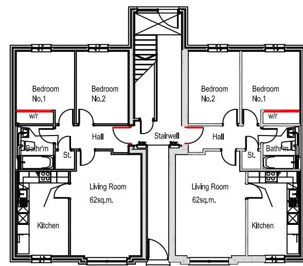
Ground Floor Plan - Standard Block Scale 1/100
